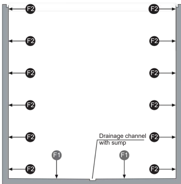
Section view
