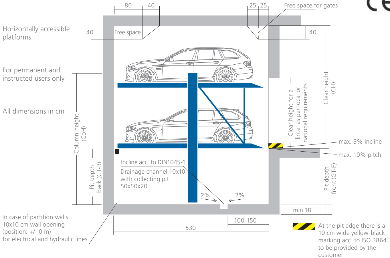
S-system for 2 cars
